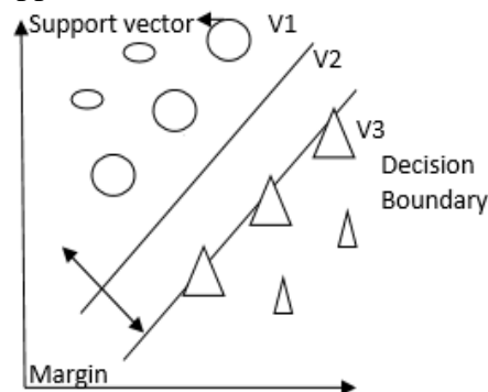
Figure 2 SVM classification
